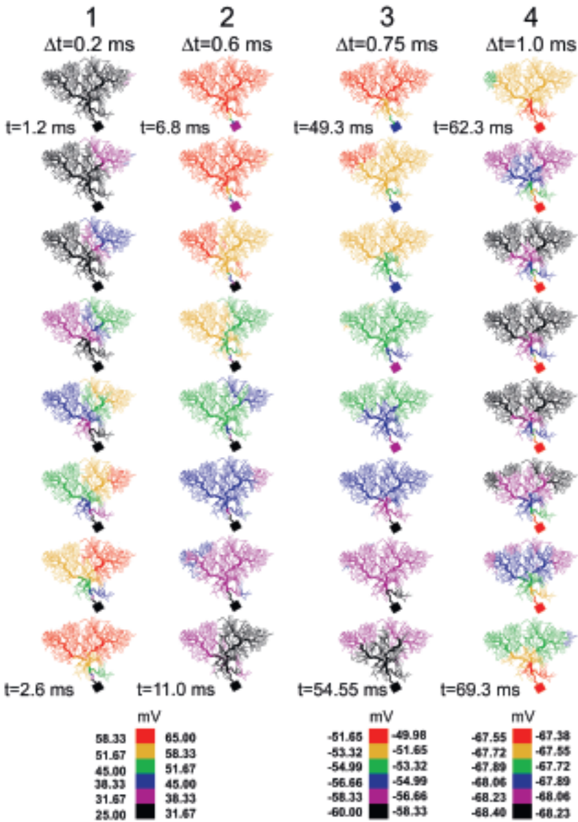
Fig. 6 - Dynamics of the electrical states of the membrane of the Purkinje cell arborization. Snapshots of the dendritic maps of the membrane potentials taken during phase 1 to 4 of the oscillatory cycle shown under the potential in Figure 5 B. Column 1 to 4 shows eight snapshots taken with equal time step \Delta t from top to bottom. Column 1 corresponds to the rising phase of the potential, starts at t=1.2 ms, snapshots taken every 0.2 ms and ends at t=2.6 ms. Column 2 corresponds to the falling phase of the plateau potential, starts at t=6.8 ms, snapshots taken every 0.6ms and ends at t=11.0 ms. Column 3 and 4 correspond to increasing ( \Delta t=0.75 ms) and decreasing ( \Delta t=1.0 ms) inter-plateau hyperpolarizations starting at t=49.3 ms and 62.3 ms and ending at t=54.55 ms and t=69.3 ms respectively. Membrane potential is colour coded in mV : from 25.00 to 65.00 mV for columns 1 and 2, from -49.98 to 60.00 mV for column 3 and from -67.38 to -68.40 mV for column 4. Note that the different scales of colour used for the different rows express different scales of voltages.
