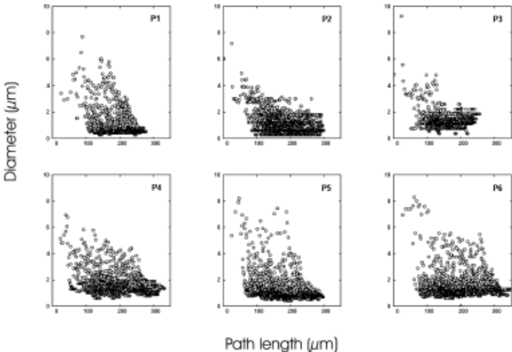
Fig. 2. - Analysis of the distribution of the dendritic diameters in the six Purkinje cells P1 to P6 identified in Material and Methods .
