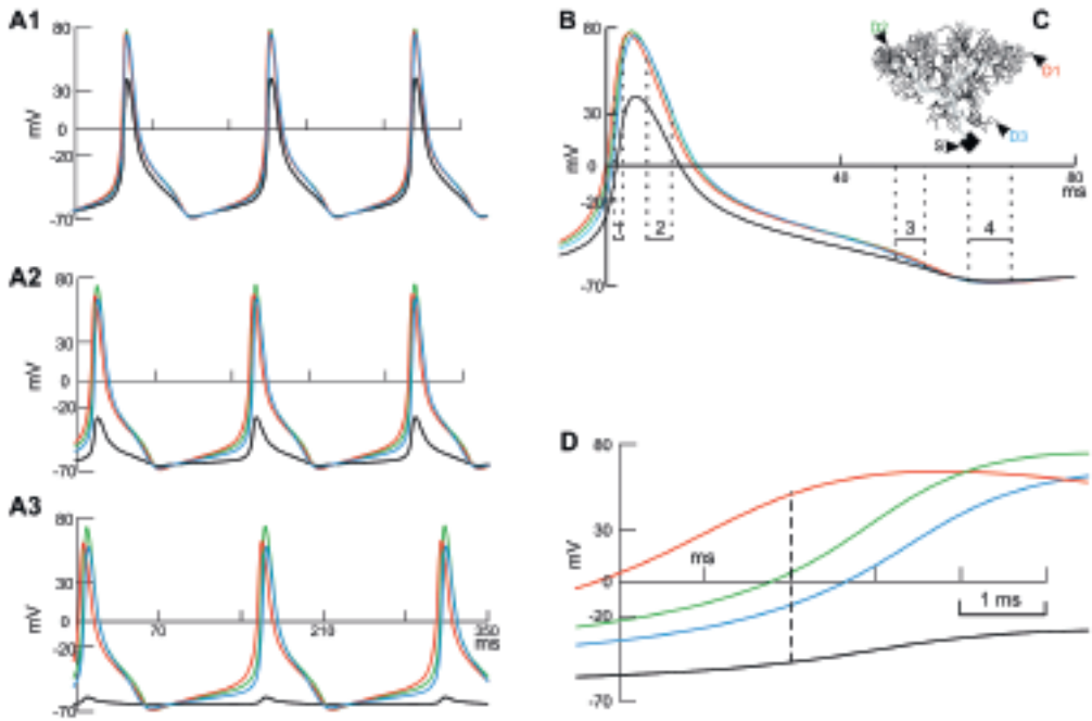
Fig. 5. - Oscillatory potentials generated by the Purkinje cell receiving distributed tonic synaptic excitation.
