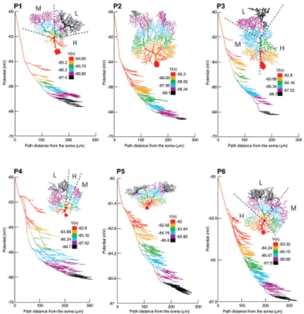
Fig. 4. - Partition of the dendritic fields into several electrical sectors observed in Purkinje neurons. Electrotonic structures of the passive dendritic arborization of six Purkinje cells, P1 to P6, identified in Material and Methods. For each cell, the voltage along the profiles (ordinates) is expressed in mV as a function of the physical distance x from the soma (abscissae) in \mu\text{m} . The colour-painted profiles indicate voltages according to each colour-scale ( V(x) ) in mV. In inset: the corresponding map of the 3D reconstructed Purkinje neuron, painted with the same colour-scale, to locate the different dendritic sectors characterized by the same voltage. In P1, P3, P4, P6 the domains looked like planar sectors approximately limited by radii (dashed lines) emerging from major branching points. In each case, sectors of low (L), medium (M), and high (H) depolarization/effectiveness are identified. In P2 and P5, the partition of the dendritic fields appears more patchy.
