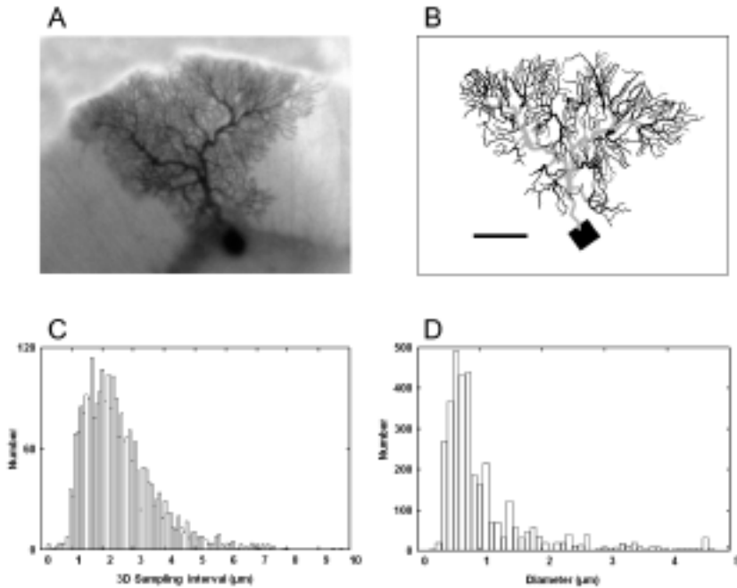
Fig. 1. - Quantitative geometry of the Purkinje cell.
