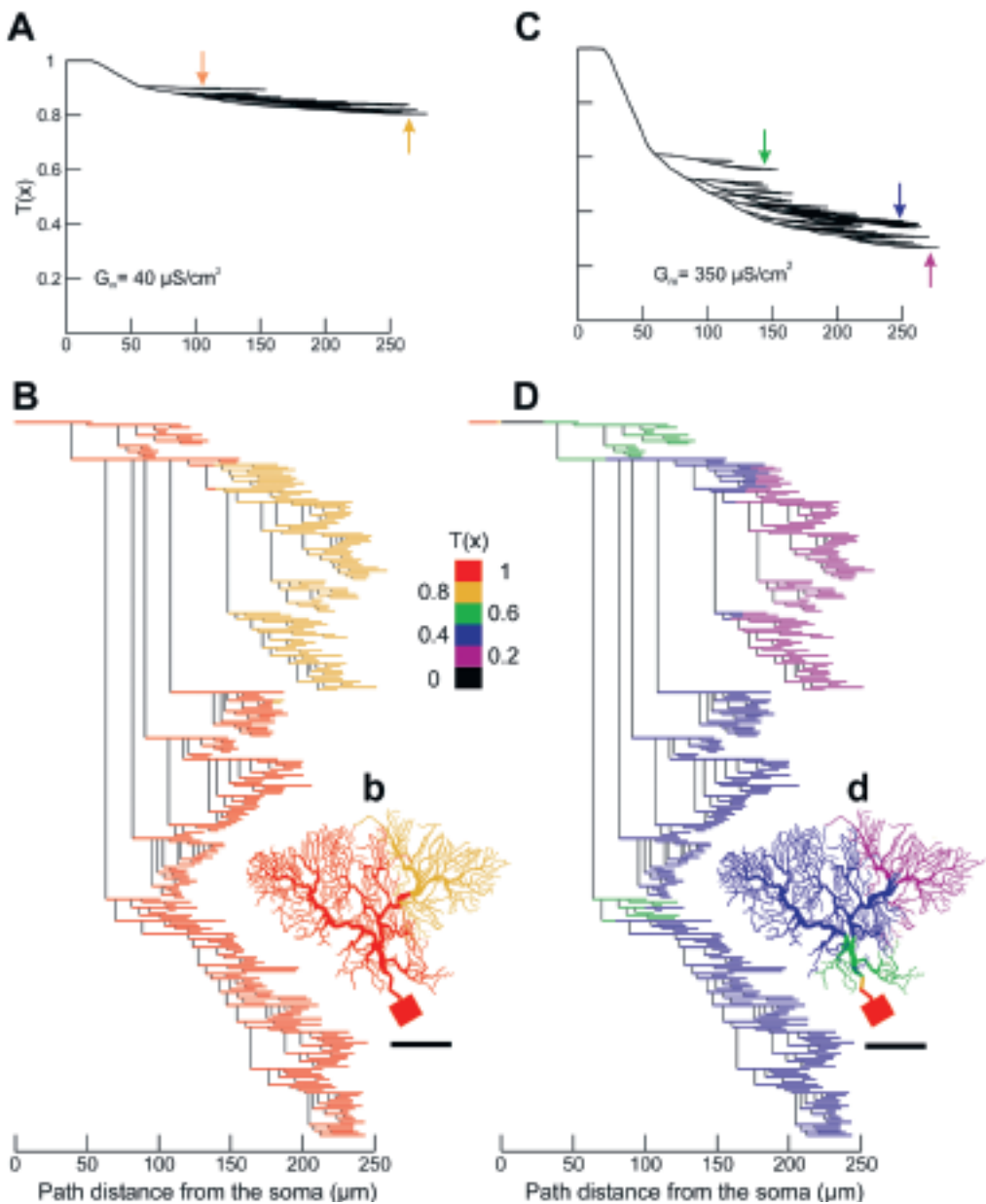
Fig. 3. - Electrotonic structure of the passive arborization of the Purkinje cell P1.
