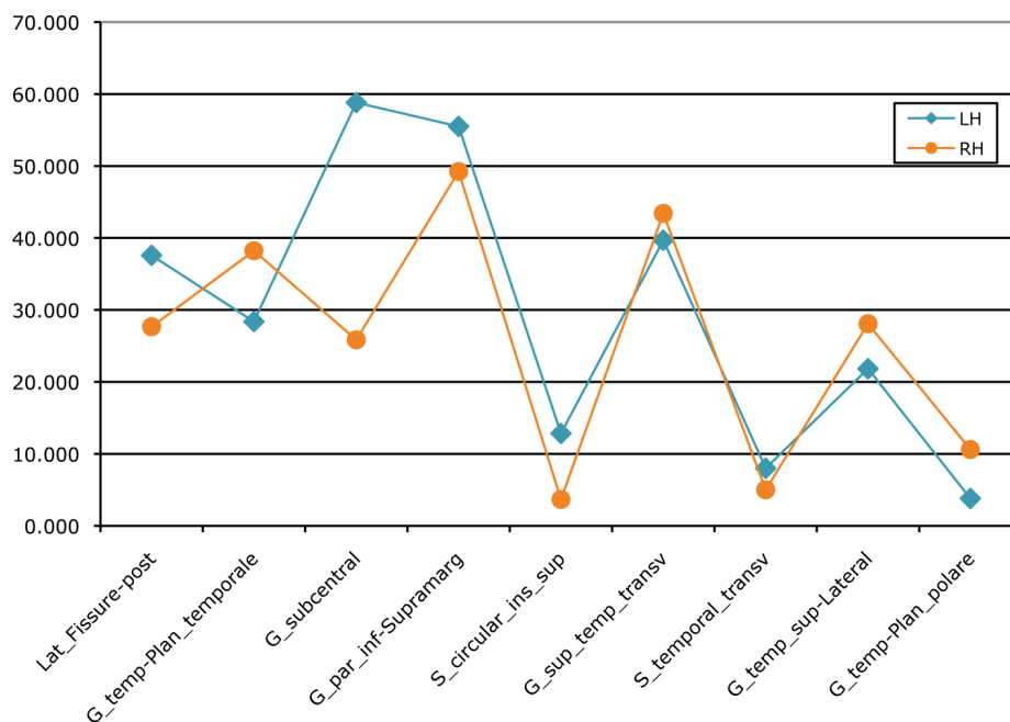
Fig. 10. - Distribution of Sylvian fissure within the lesion: Comparison of average number of voxels from all subjects (Y axis) per Freesurfer labels (x axis) between the right and left hemispheres in the Sylvian fissure which was affected by the stroke in all participants. Note the close parallels between the Freesurfer profile in the right and left hemispheres.
