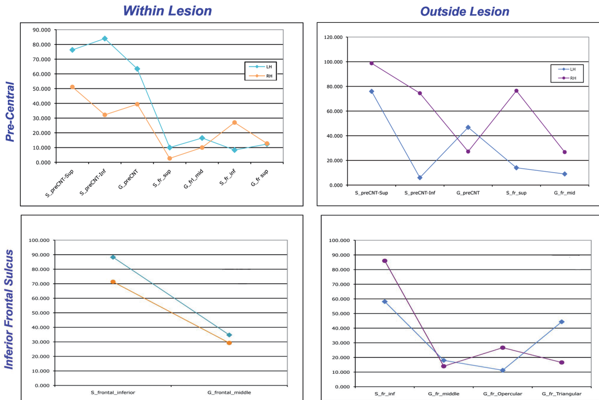
Fig. 9. - The case of frontal sulci: Comparison of average number of voxels from all subjects (Y axis) per freesurfer classifications (x axis) between the right and left hemispheres in the inferior frontal and the precentral sulci. The left column represent the cases affected by the stroke, the right column, the same sulci when not lesioned. Note the reciprocal relationship in the complexity of these sulci which tend to be some of the most variable in the brain.
